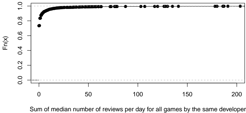
Fig. 4: The empirical cumulative distribution function ( F_n(x) ) of the sum of median numbers of reviews per day for all games developed by the same developer
