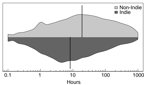
Fig. 15: The distributions of playing hours that are associated with reviews for indie and non-indie games. The vertical lines represent the median. The distributions are significantly different ( p < 0.05 ), with a small effect size.
