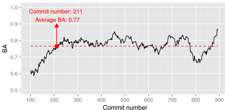
Fig. 5 The balanced accuracy of the within-project classifiers for HttpClient
