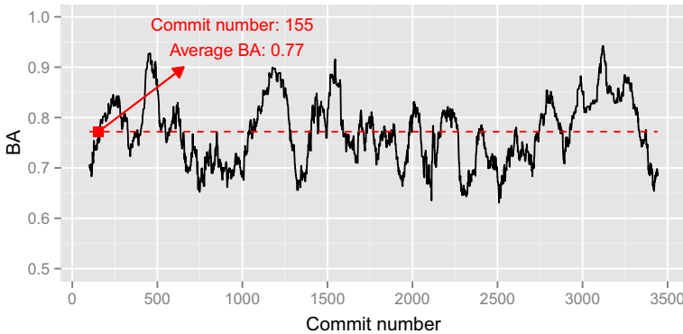
Fig. 6 The balanced accuracy of the within-project classifiers for Qpid
